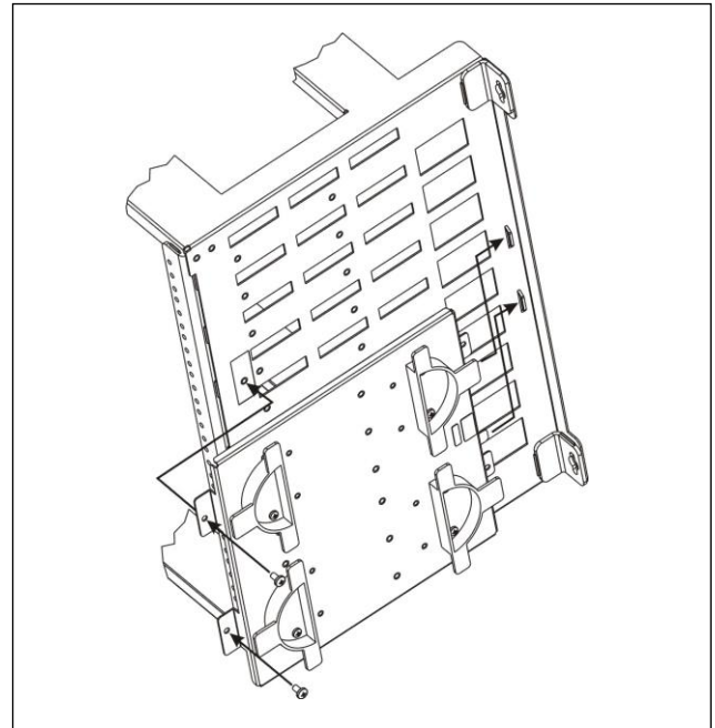
Figure 10. SPL-4H installation
