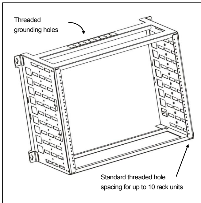
Figure 3. WR-10U23 Features
