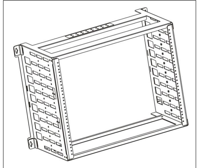
Figure 1. WR-10U23 Wall Rack
