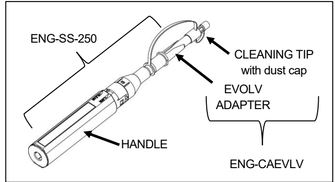
Figure 1. ENG-SS-250 cleaning tool with ENG-CAEVLV installed
