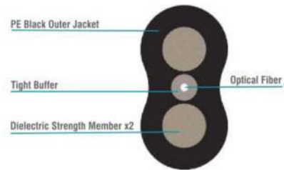
Micro-Flat Drop Cable 3mm x 5.4mm (0.12" x 0.21") Non-toneable shown
