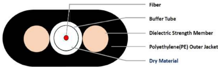
Standard Flat Drop Cable 4.5mm x 8mm (0.18" x 0.315") Dry, non-toneable shown
