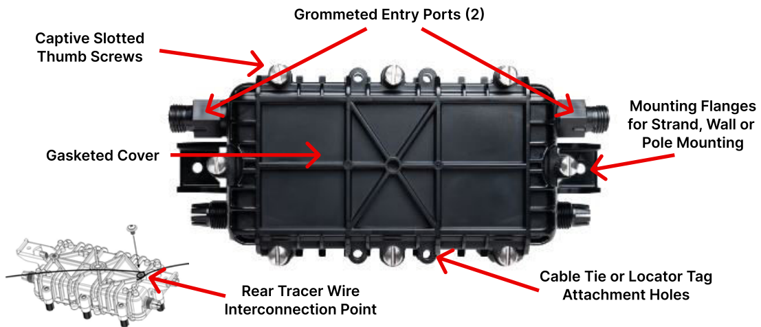
LOC-DROP Housing—Exterior
