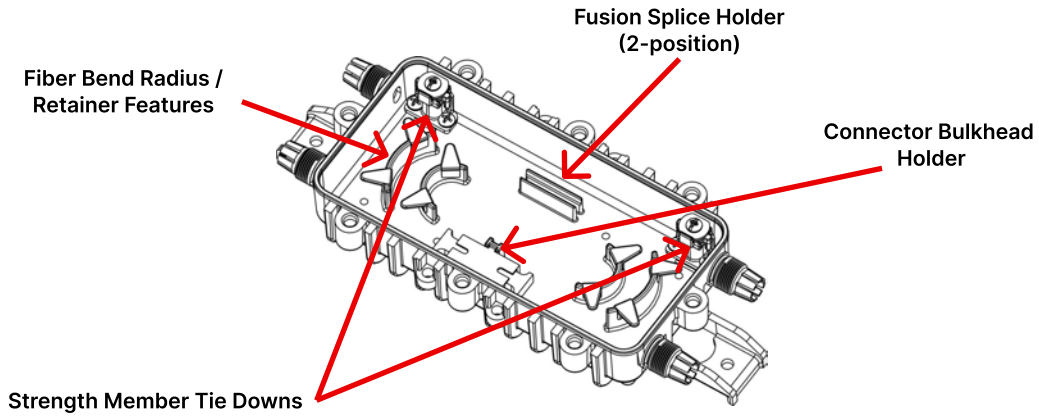
LOC-DROP Housing—Interior
