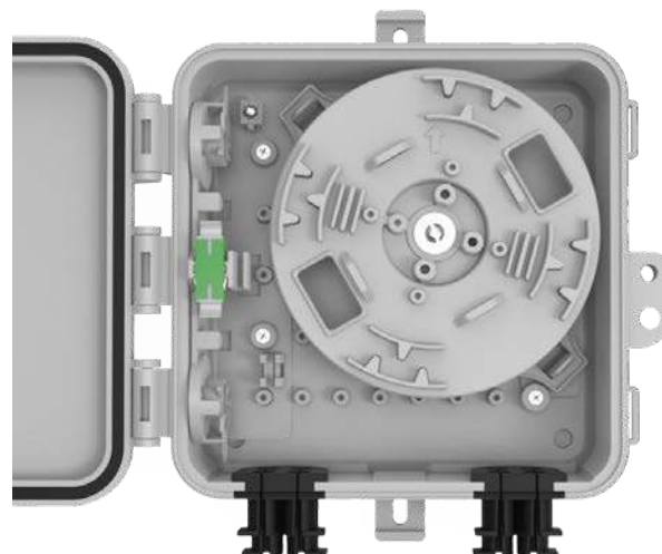
Spool NID with Fiber Spool installed. Fiber Spool sold separately.
